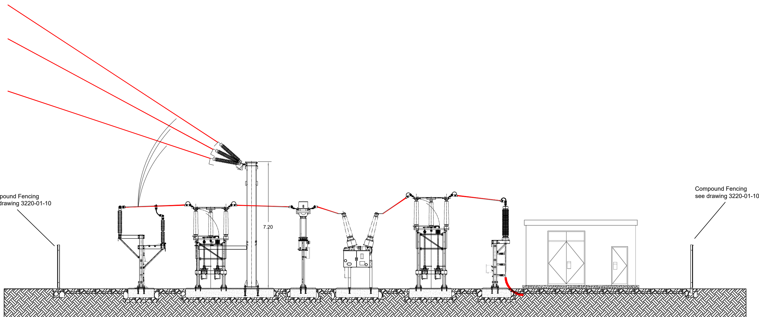
Surge Arrester / Post Insulator Disconnecter Gantry CT/VT Circuit Breaker Disconnecter Cable Sealing End DNO Substation (see drawing 3220-01-9b)
