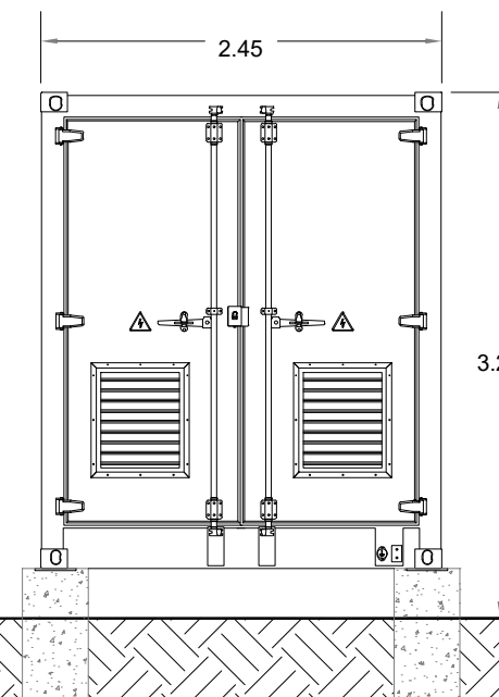
SIDE ELEVATION
