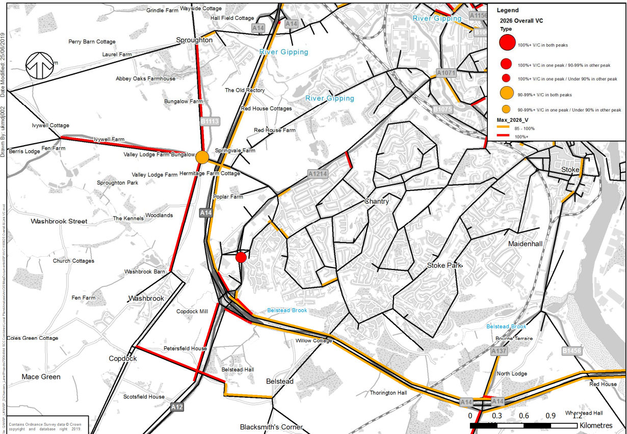
Figure 13 – West / South West of Ipswich – 2026 Links and Junctions with V/C 85%+ - No Adjustment
