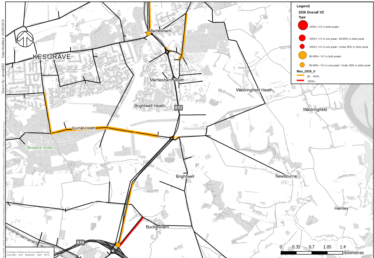
Figure 5 – A12 East of Ipswich – 2026 Links and Junctions with V/C 85%+ - No Adjustment
