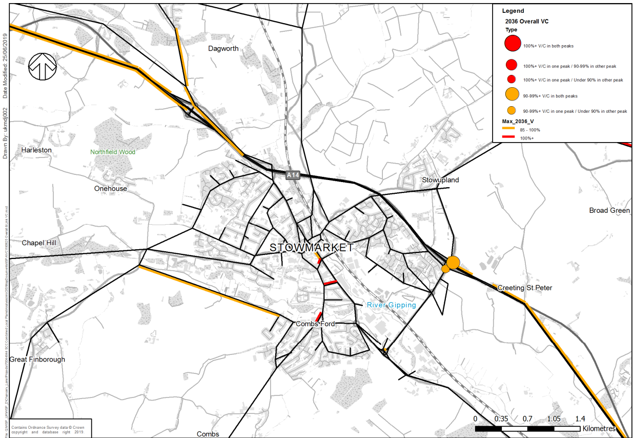
Figure 22 – Stowmarket – 2036 Links and Junctions with V/C 85%+ - No Adjustment
