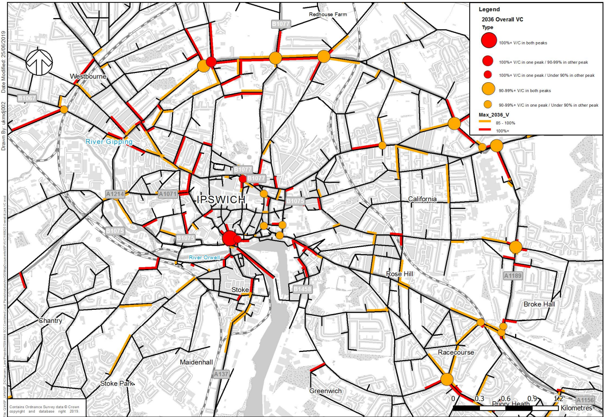
Figure 12 – Ipswich – 2036 Links and Junctions with V/C 85%+ - No Adjustment
