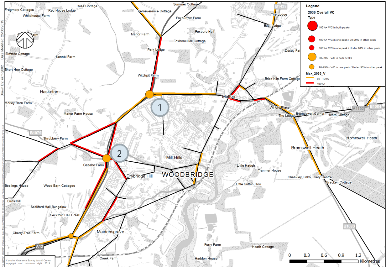
Figure 4 – Woodbridge & Melton – 2036 Links and Junctions with V/C 85%+ - No Adjustment
