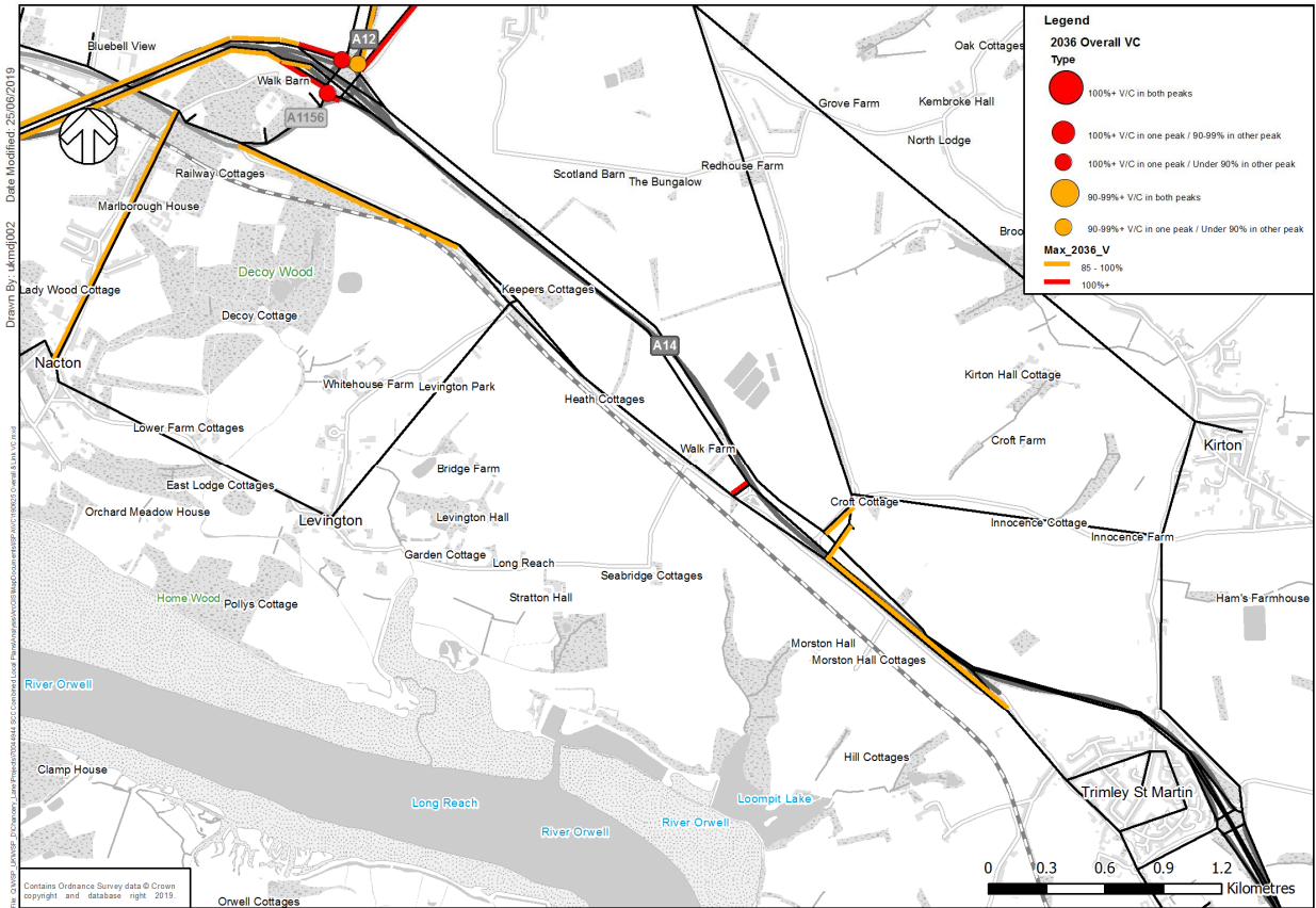
Figure 10 – Nacton to Trimley St. Martin – 2036 Links and Junctions with V/C 85%+ - No Adjustment
