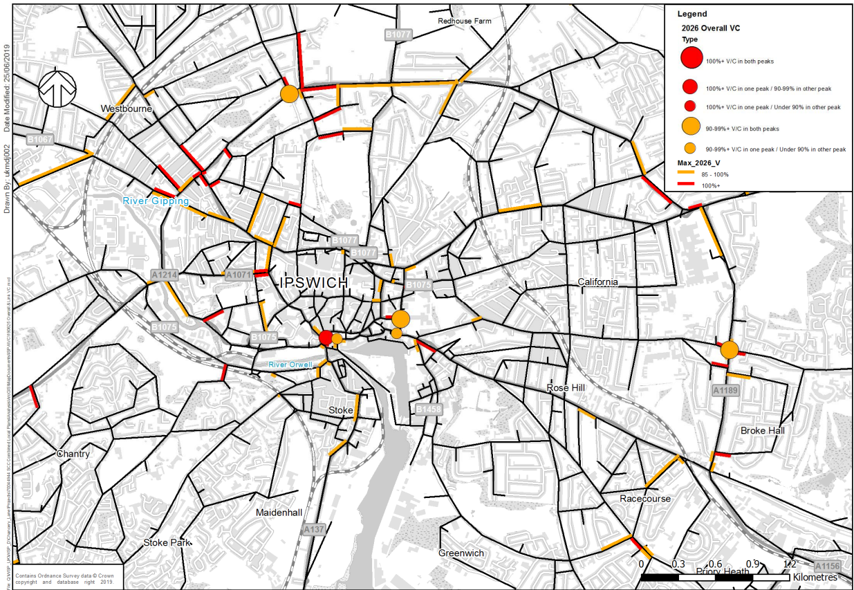
Figure 11 – Ipswich – 2026 Links and Junctions with V/C 85%+ - No Adjustment
