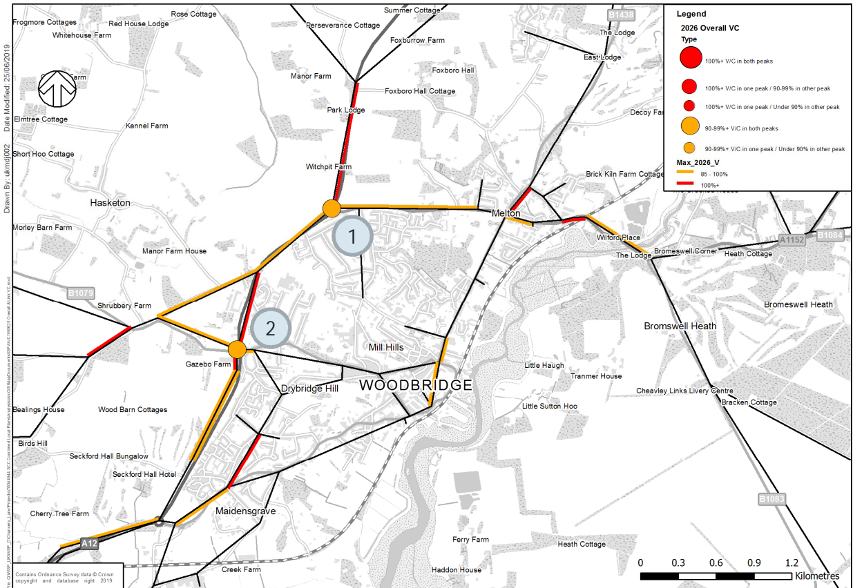
Figure 3 – Woodbridge & Melton – 2026 Links and Junctions with V/C 85%+ - No Adjustment
