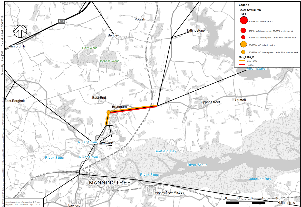
Figure 17 – Brantham – 2026 Links and Junctions with V/C 85%+ - No Adjustment
