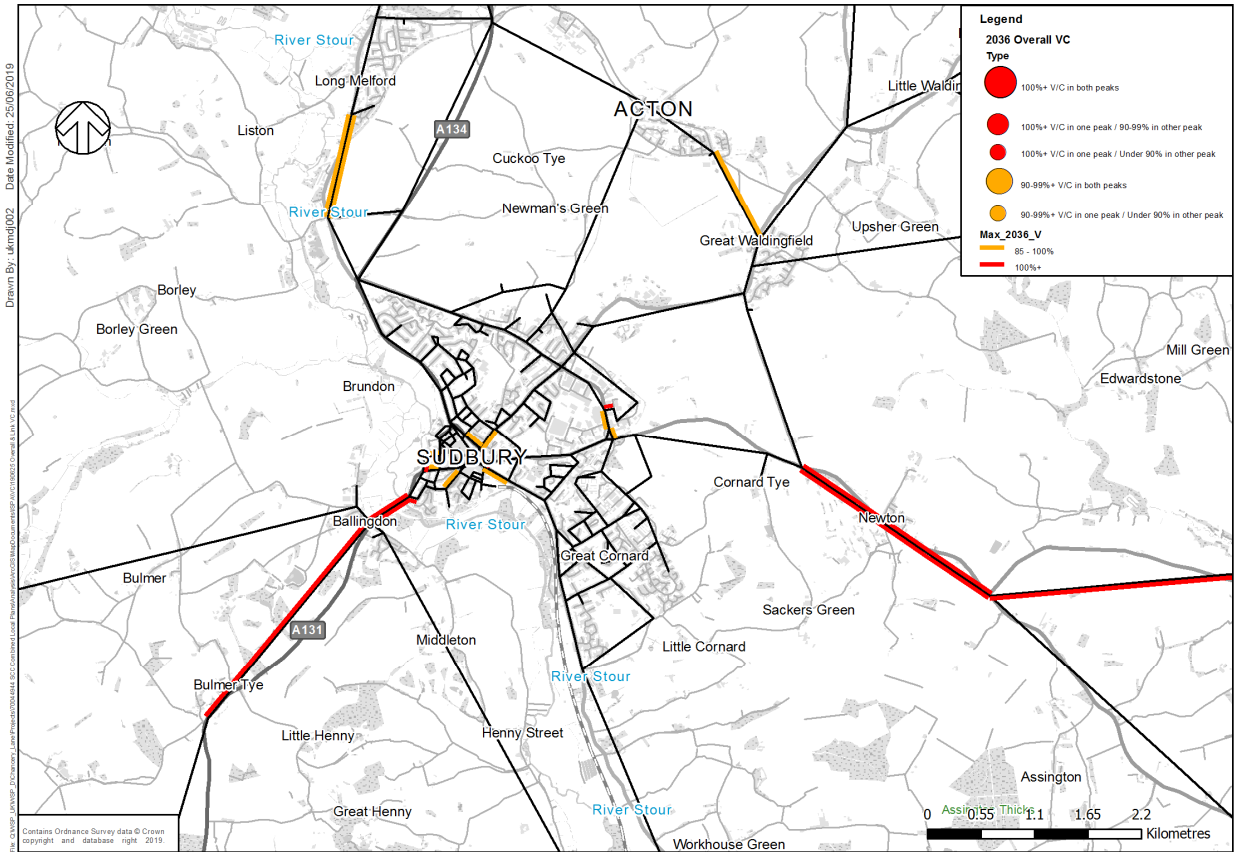
Figure 16 – Sudbury – 2036 Links and Junctions with V/C 85%+ - No Adjustment
