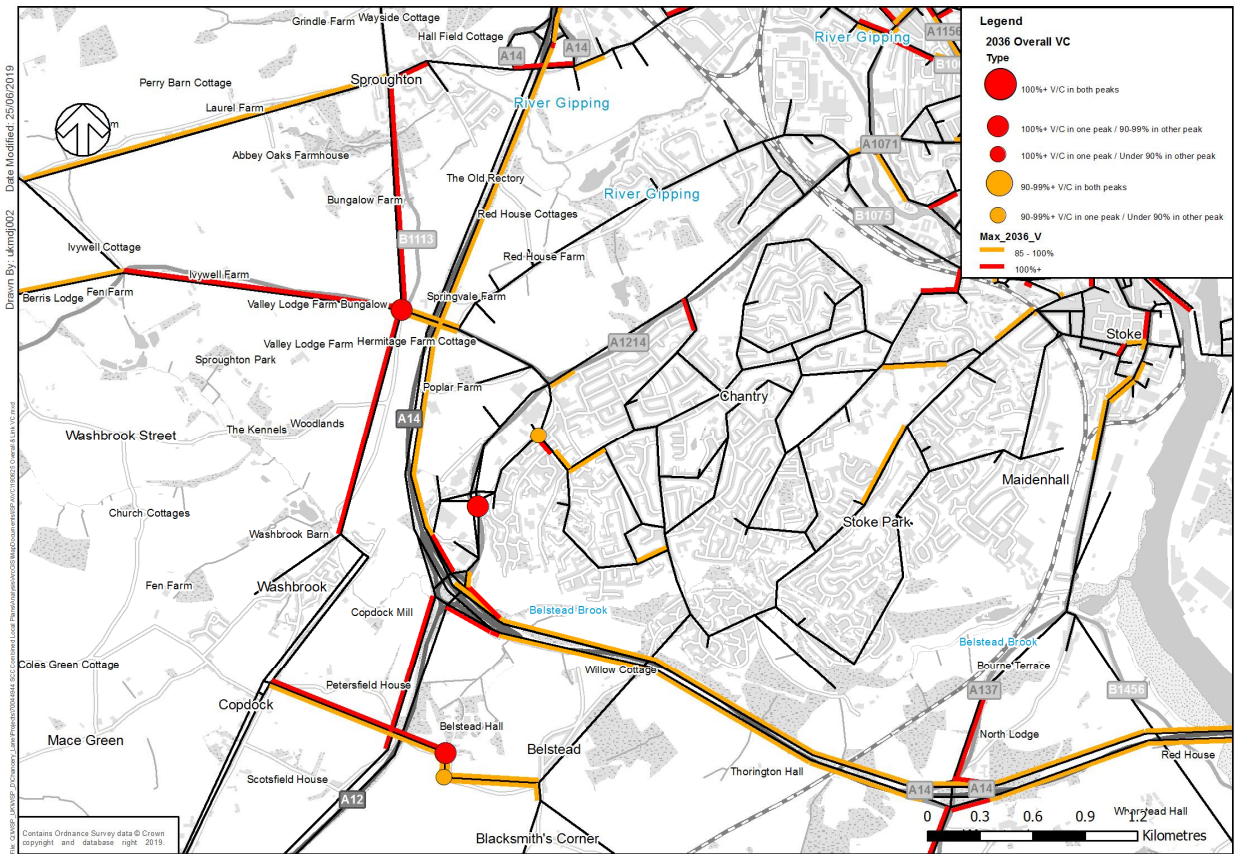
Figure 14 – West / South West of Ipswich – 2036 Links and Junctions with V/C 85%+ - No Adjustment
