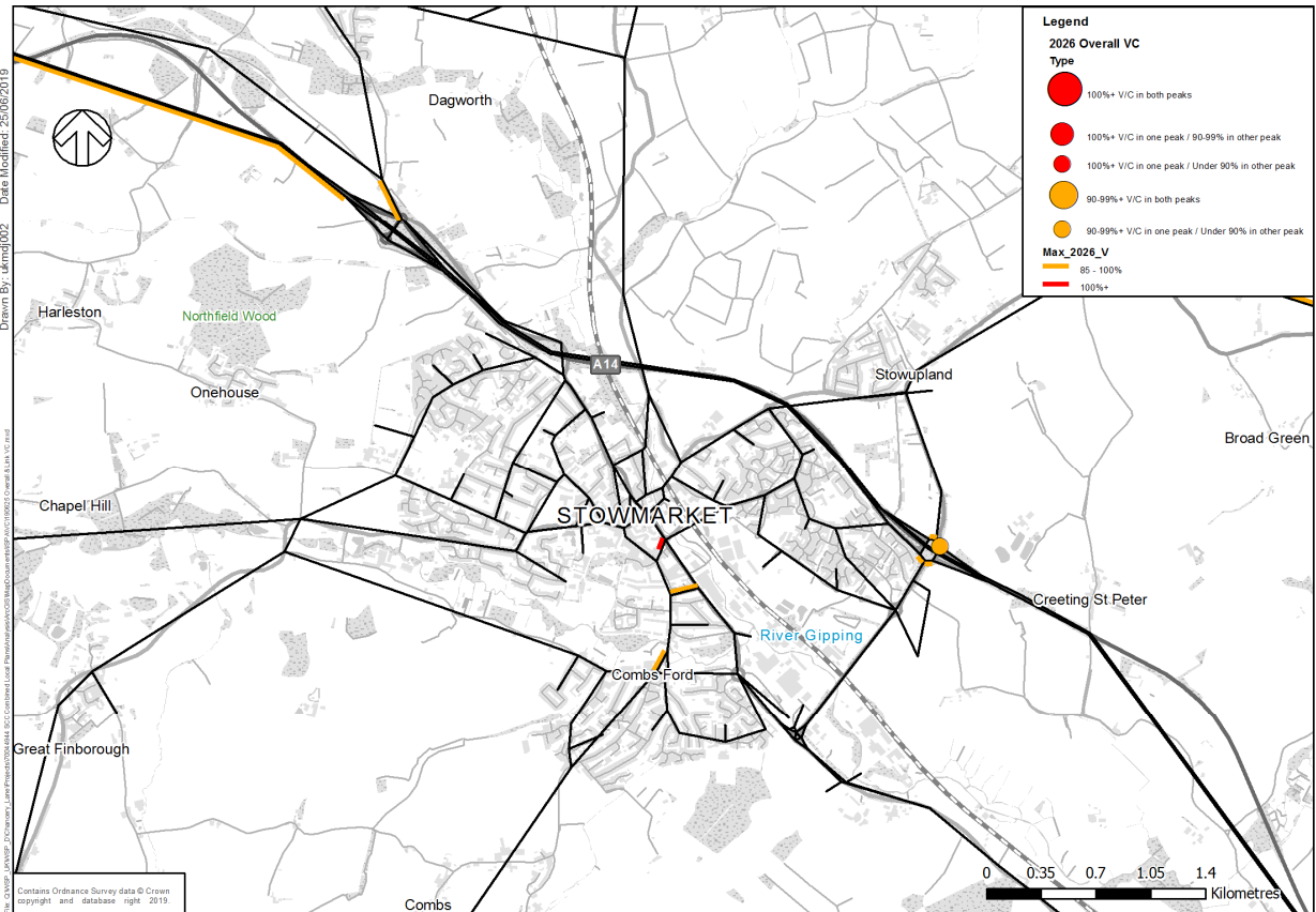
Figure 21 – Stowmarket – 2026 Links and Junctions with V/C 85%+ - No Adjustment
