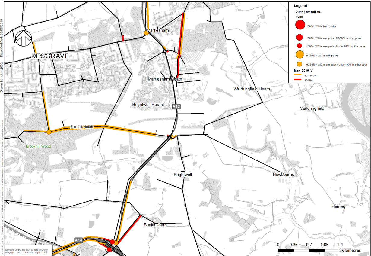
Figure 6 – A12 East of Ipswich – 2036 Links and Junctions with V/C 85%+ - No Adjustment
