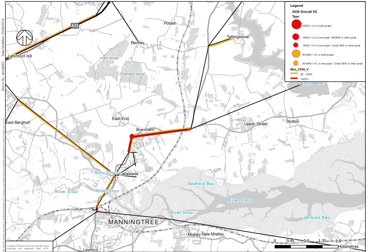
Figure 18 – Brantham – 2036 Links and Junctions with V/C 85%+ - No Adjustment
